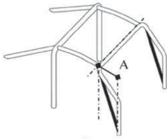
R Reinforcement between main hoop and floor attachment point of front hoop dwg. 253-15
