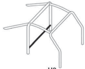
H3 Wrap around harness attachment bar dwg. 253-30
