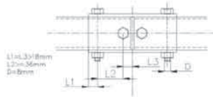
S Sleeve connecting tubes dwg. 253-41
